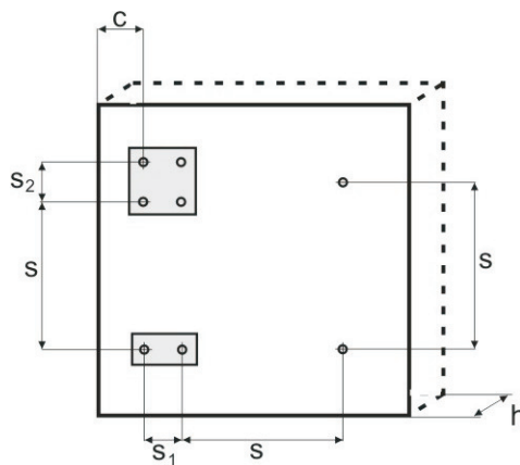
Scheme of distance and spacing in masonry ( use category “b” and “c”)
