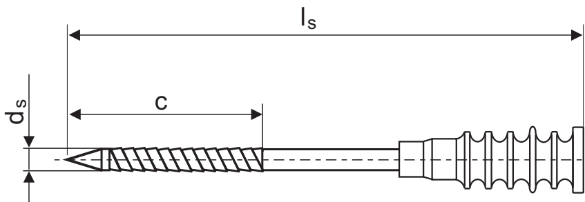
Nail with an integrally moulded plastic head
